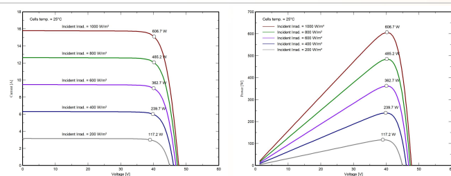
Current-Voltage Characteristic
